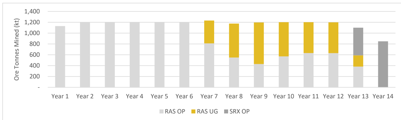
Figure 1 Ore Feed Schedule 1.2Mtpa
