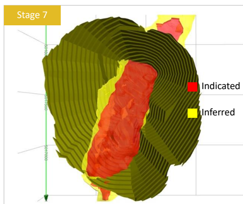
Figure 10 Pit Shells w/Ramps Showing IND/INF
