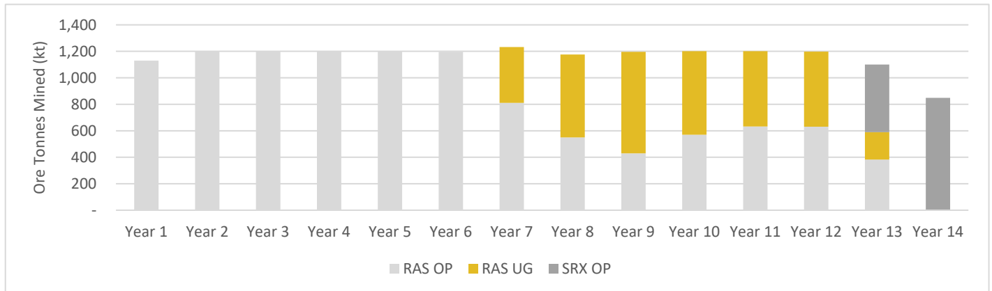
Figure 15 Open Pits vs Underground Mill Feed
