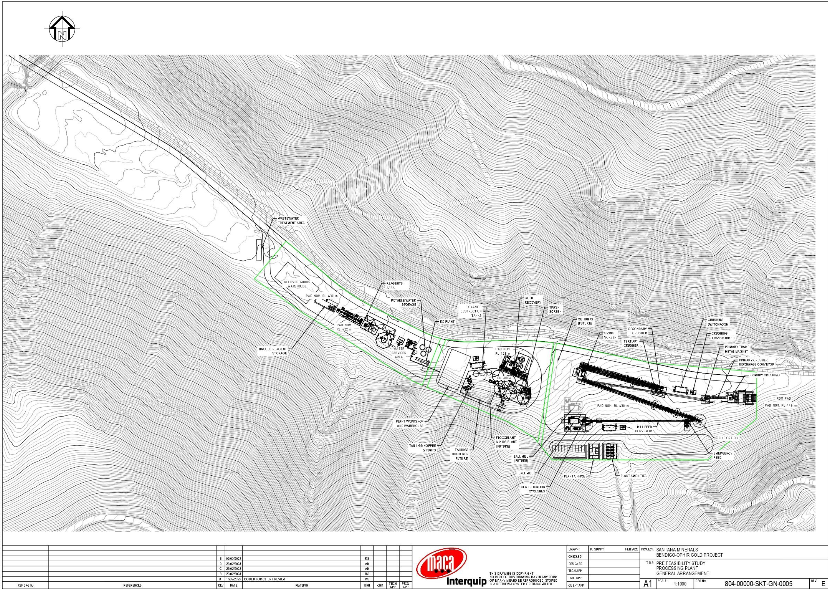
Figure 17 General Arrangement Drawing of BOGP Processing Plant
