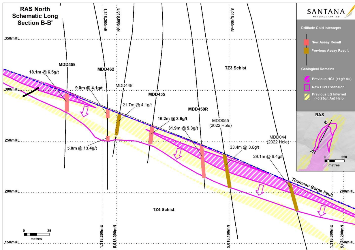
Figure 3. RAS North Oblique Long Section Showing Down Plunge Grade Continuity
