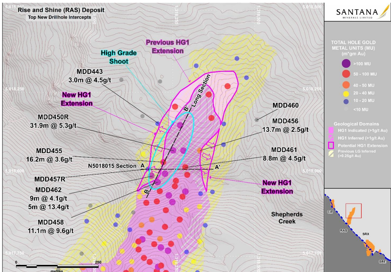
Figure 1. Plan View of RAS North Drilling Showing Potential HG1 Extension
