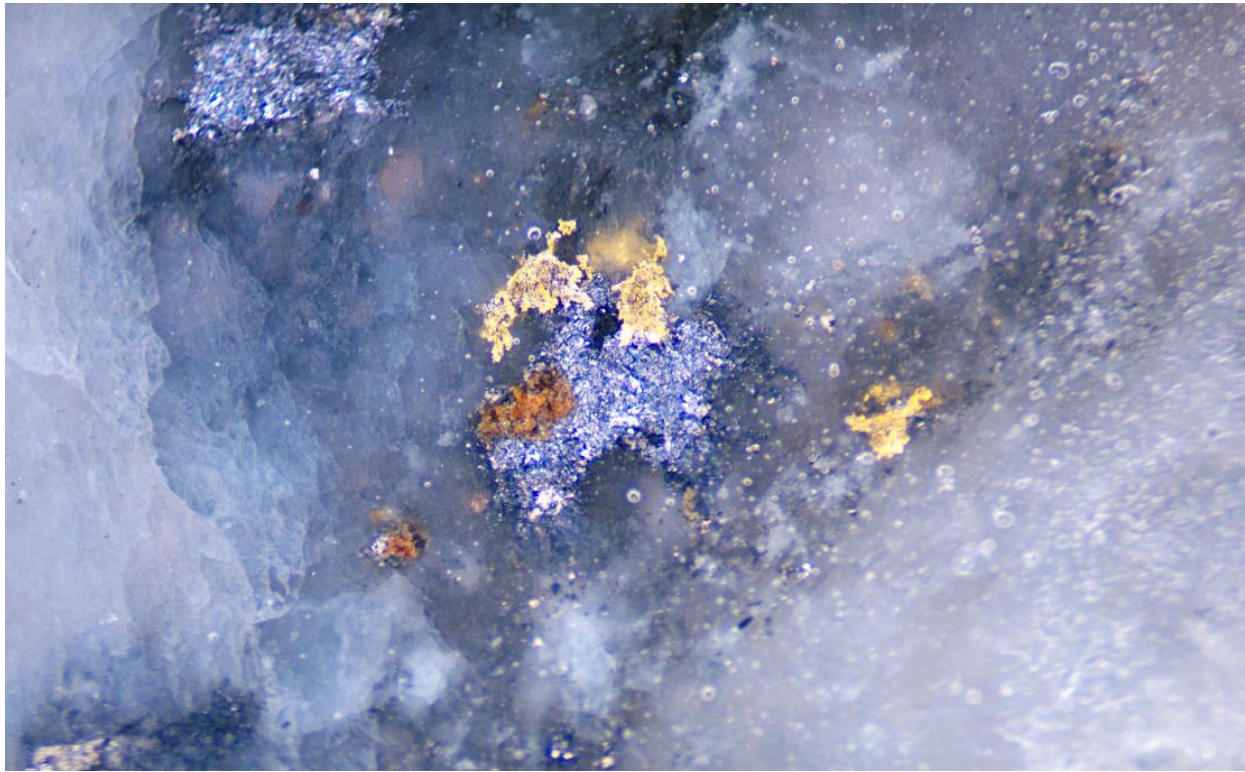
Figure 4. Visible Gold in MDD450R at 306.7m
