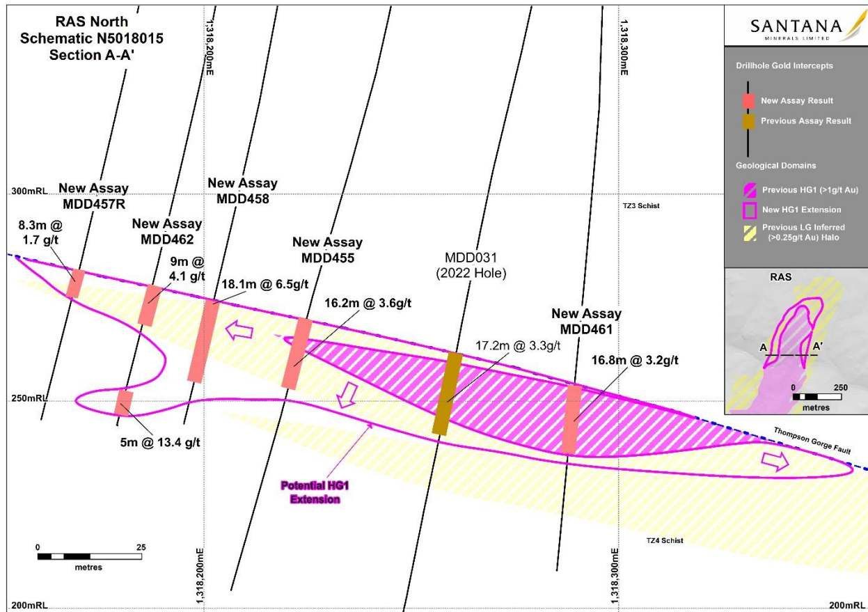
Figure 2. RAS North EW X-Section N5018015 Showing Potential Extension of HG1 Domain Thickness
